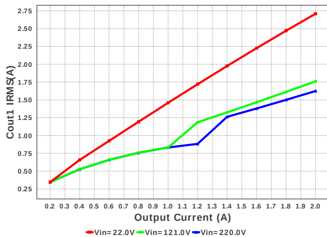
Cout1 IRMS(A)
